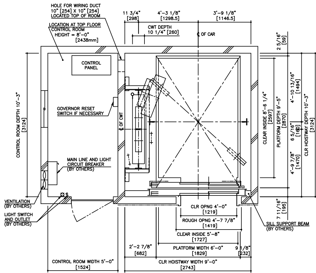
HOISTWAY PLAN WITH CWT SAFETY
