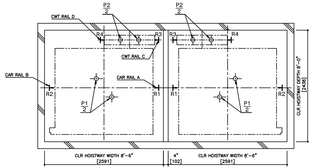
PIT PLAN WITHOUT CWT SAFETY
