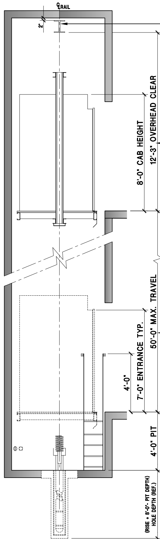
HOISTWAY SECTION
