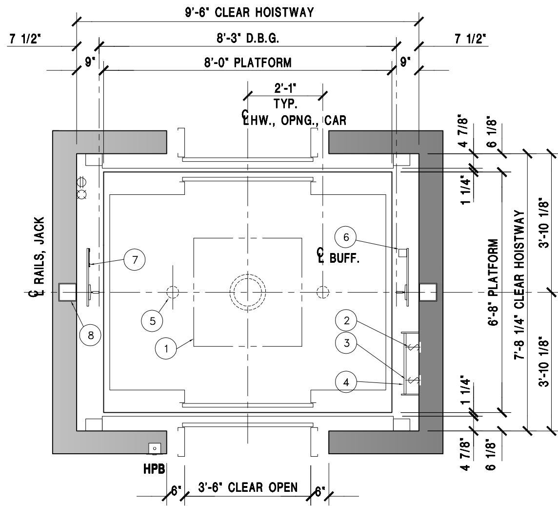
HOISTWAY PLAN
