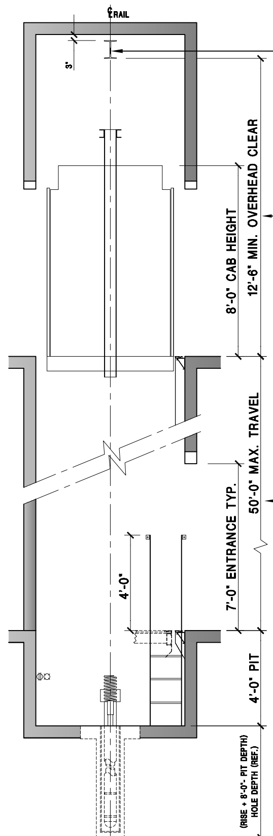
HOISTWAY SECTION
