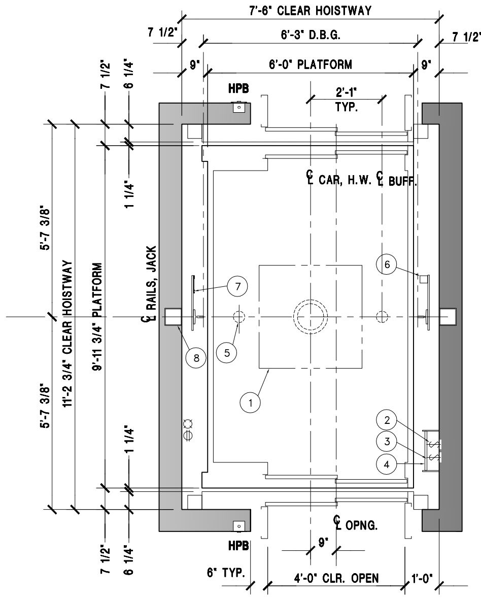
HOISTWAY PLAN
