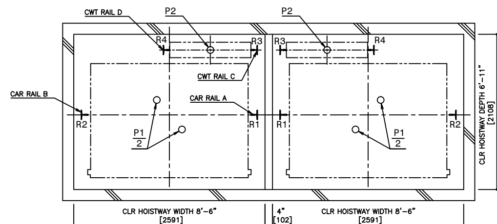
PIT PLAN WITHOUT CWT SAFETY
