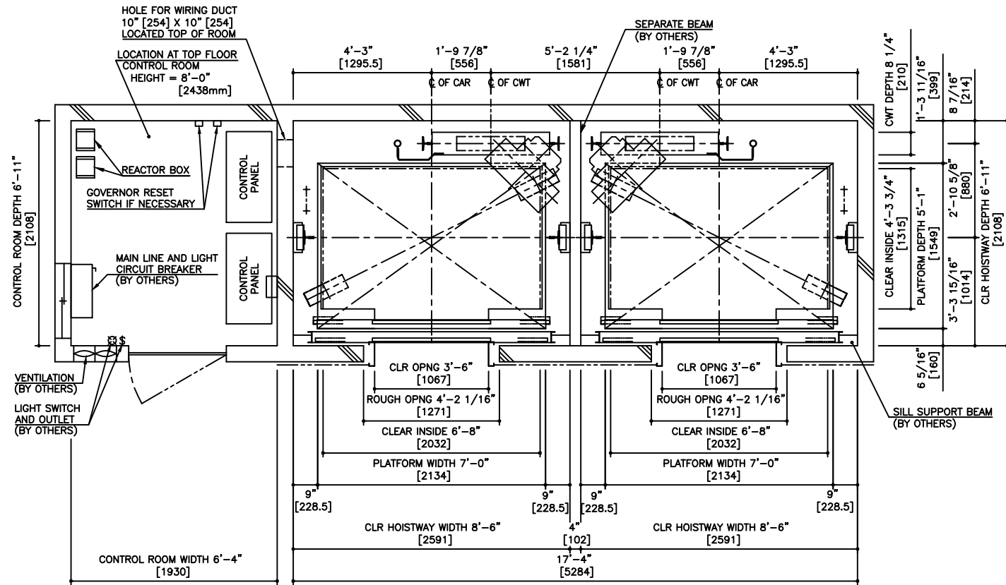
HOISTWAY PLAN WITHOUT CWT SAFETY
