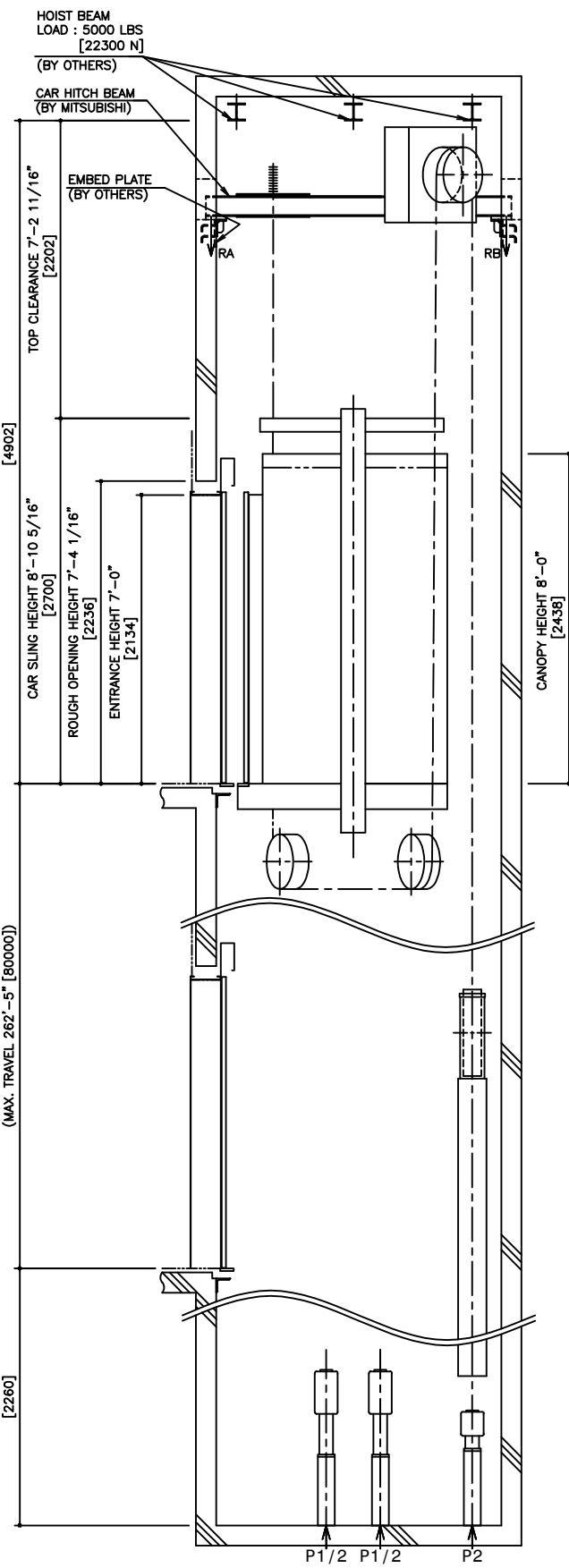
HOISTWAY SECTION WITHOUT CWT SAFETY
