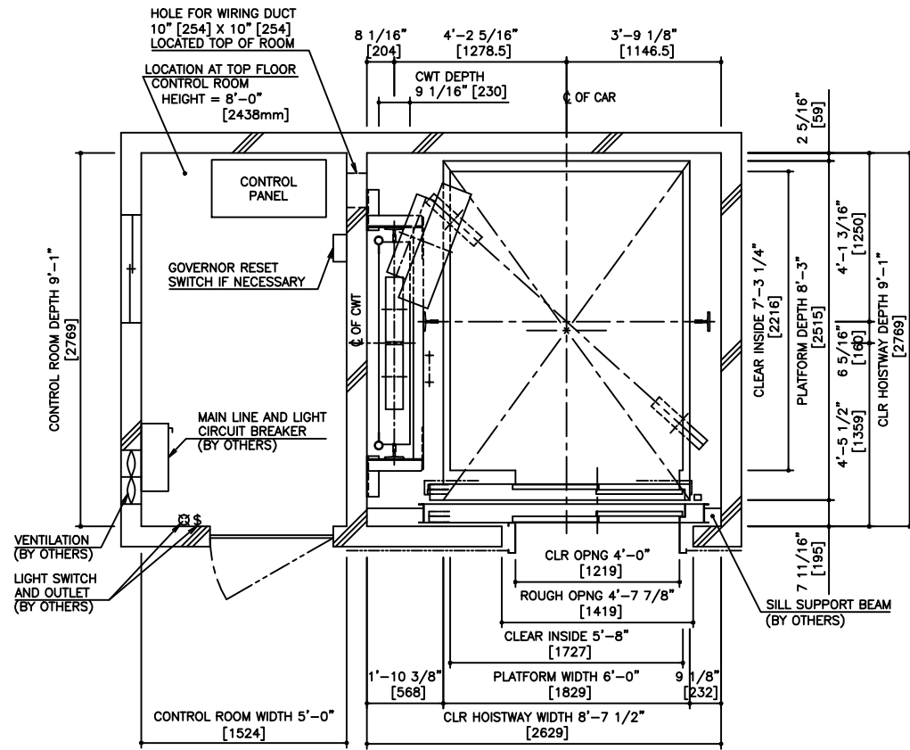
HOISTWAY PLAN WITHOUT CWT SAFETY
