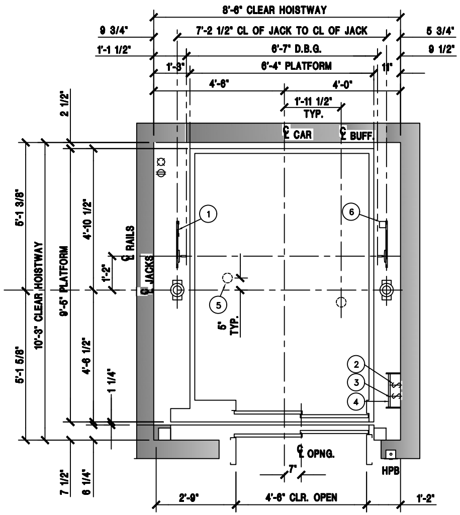
HOISTWAY PLAN
