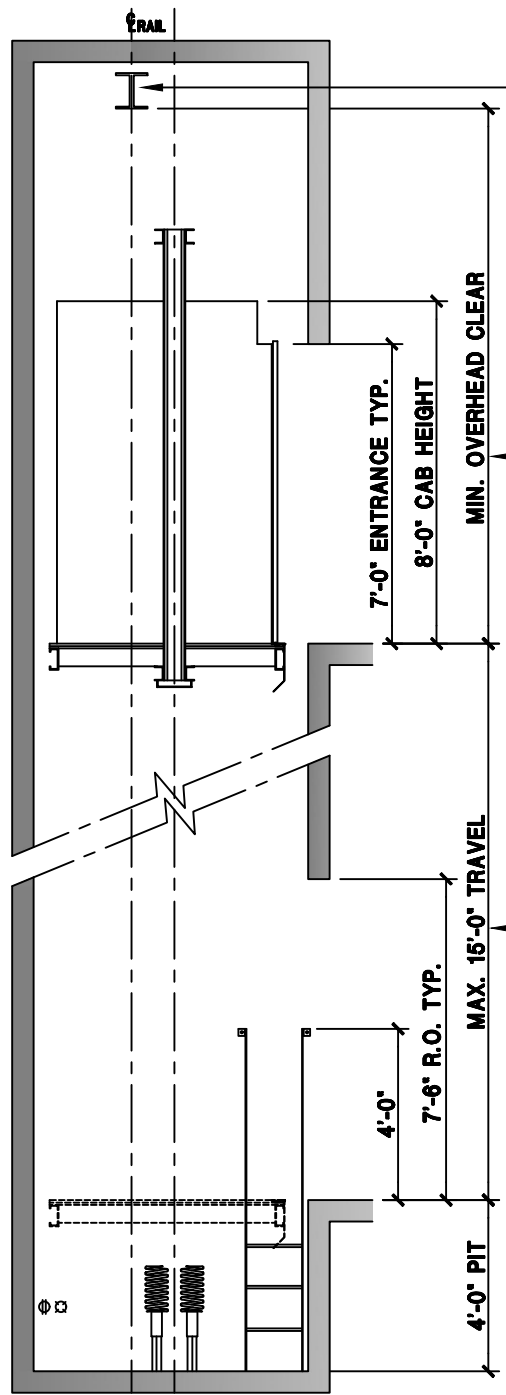
HOISTWAY SECTION
