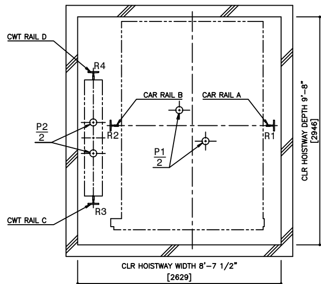
PIT PLAN WITHOUT CWT SAFETY
