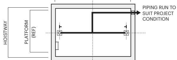
Plan View of Elevator Pit Condition
