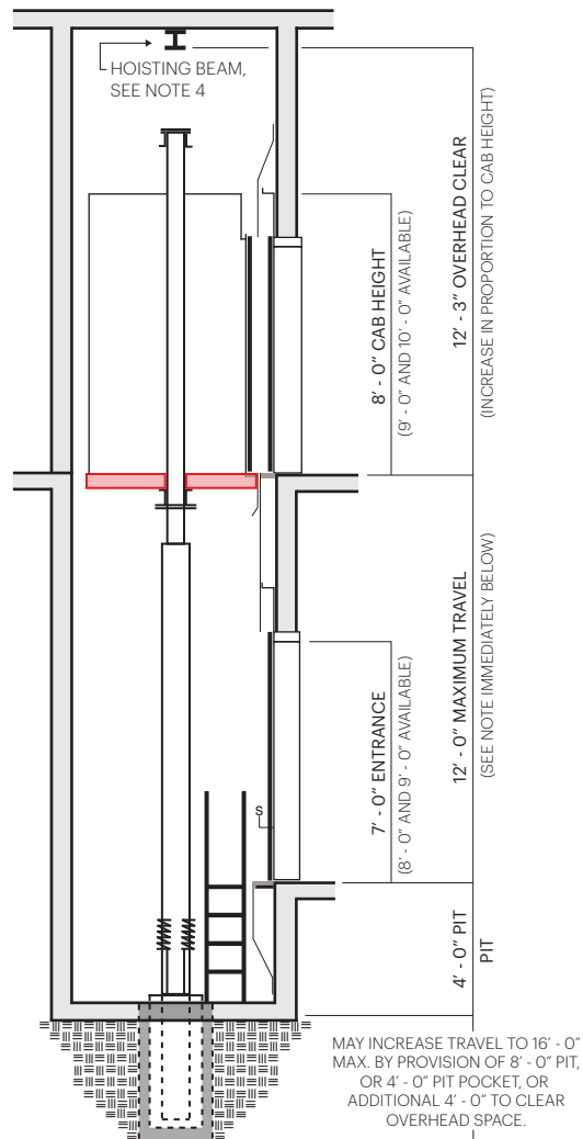
Composite Hoistway Section
