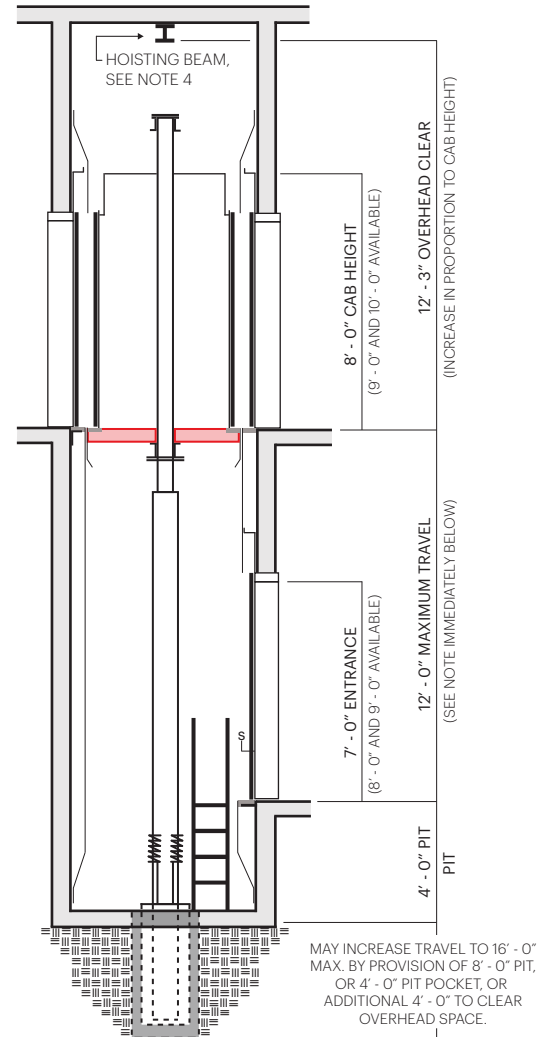
Composite Hoistway Section
