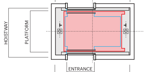
Plan View of Handed Single Slide
