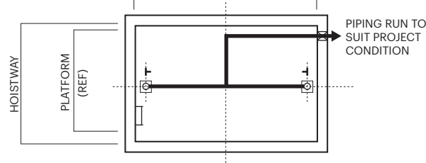
Plan View of Elevator Pit Condition
